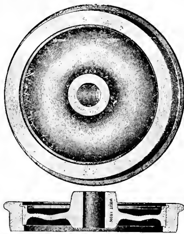
Figs. 5296-5297. WROUGHT-IRON DISC CENTER WHEEL. Brunswick Tire-fastenings.
